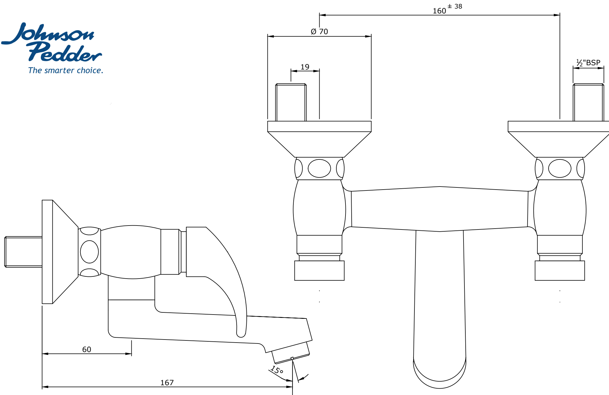
JT1241A1 Genex Hercules Wall Mixer (Non Shower)
